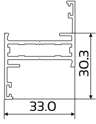
DIE No. W55691 Tubular Sash
