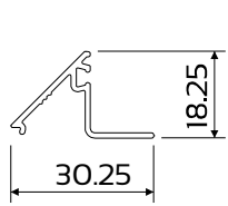
DIE No. W33137 Cas34 Bead Multi 13mm
