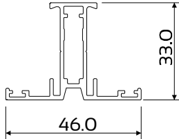
DIE No. W56271 Cas34 Mullion 34mm Cottage Pane
