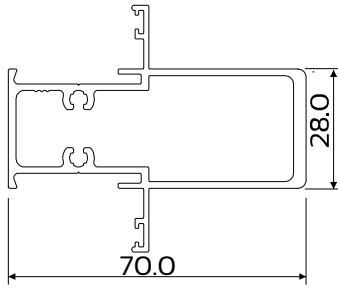
DIE No. W56270 Cas34 70mm Mullion
