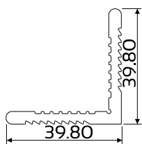
DIE No. W52538 Osborne Multi Corner Cleat
