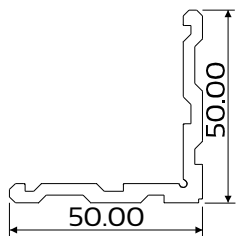
DIE No. CL10241P Cas34 Corner Cleat
