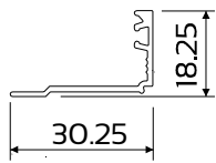
DIE No. W33136 Cas34 Bead Double Glaze
