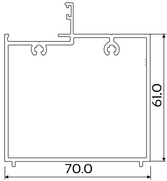
DIE No. W56272 Cas34 Frame 70mm Boxed Sill
