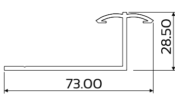
DIE No. W10627 Fixing Lug
