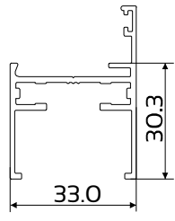
DIE No. W32039 Equal Leg Outer Frame
