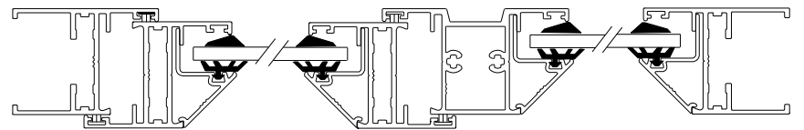
SECTION A-A Section not to scale
