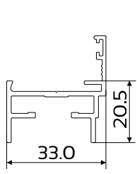
DIE No. W33134 Cas34 Frame 34mm Short Leg
