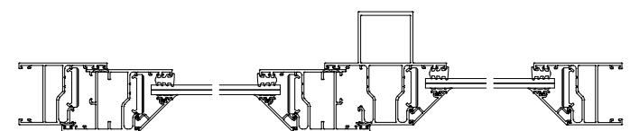
SECTION C-C
