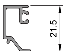
Evolution Square Bead 13 mm Gap (Still to be cut)
