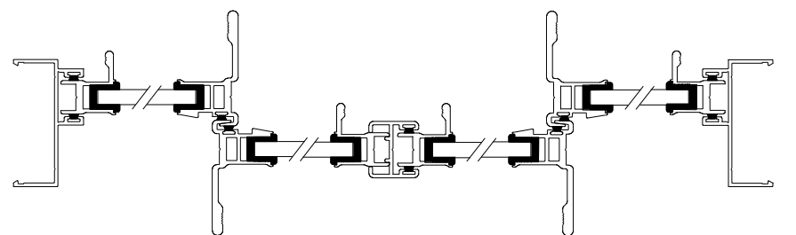
SECTION A-A Section not to scale
