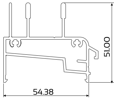
DIE No. W53322 Hollow Sill Rail
