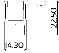
DIE No. W28476 Sash Outer Frame
