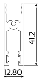
DIE No. W28475 Sash Head & Sill
