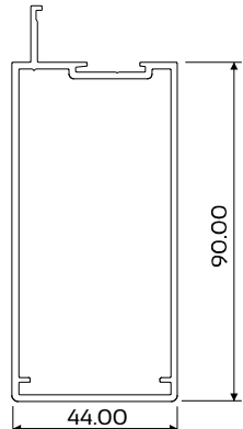
DIE No. W53406 Clip44 R9 D/Stile 90mm
