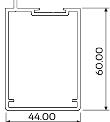
DIE No. W53099 Clip44 R11 60mm D/Stile
