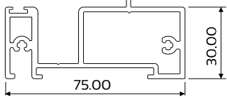
DIE No. W55113 Clip44 Head Vistafold
