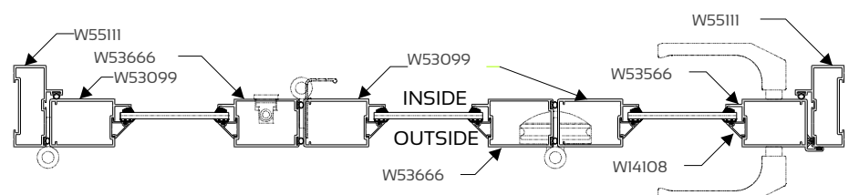
SECTION A-A Section not to scale
