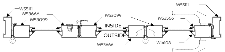
SECTION B-B Section not to scale
