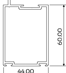
DIE No. W53666 Clip44 R1ISP D/Stile 60mm
