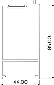
DIE No. W44088 Clip44 R4 Head/Sill Rail
