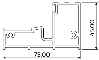
DIE No. W55112 Clip44 Sill Vistafold
