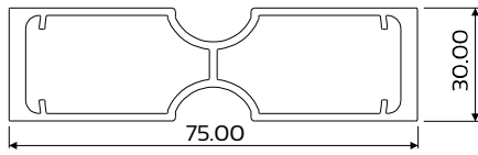
DIE No. W55563 Clip44 HD Mullion Vistafold
