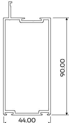
DIE No. W53407 Clip44 R9W D/Stile 90mm W/Pile
