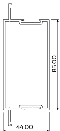
DIE No. W44089 Clip44 R4-Special Midrail 85mm
