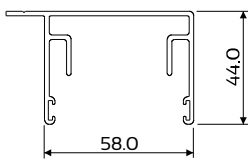
DIE No. W26198 Head Rail Top Guide
