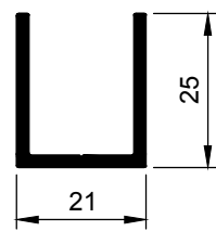
U-Channel W26152
