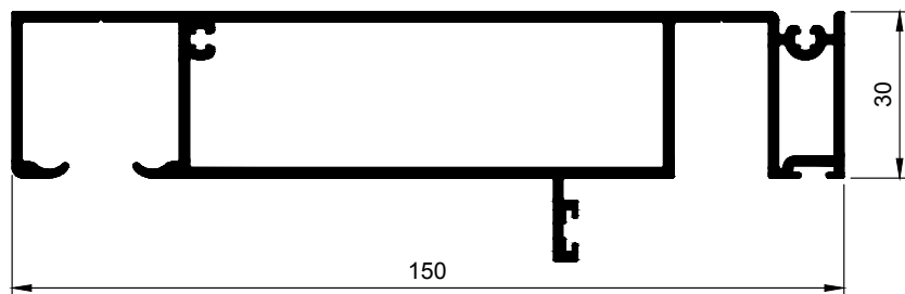
Horizon Head Rail W57567
