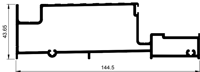
Horizon Sill Rail W57568
