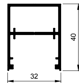
Stile 32 mm W56087
