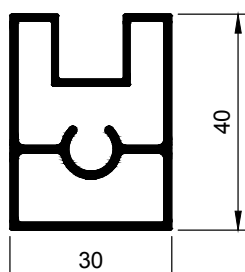
Top/Bottom 32 mm W56085
