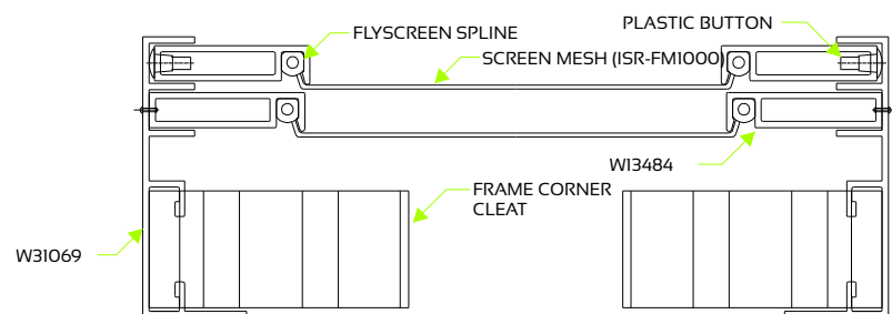
SECTION A-A Section not to scale
