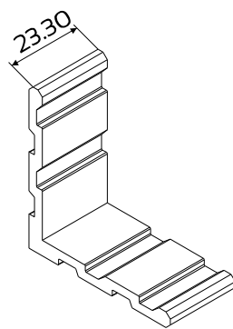
LGC-52695-28 Dusk Corner Cleat
