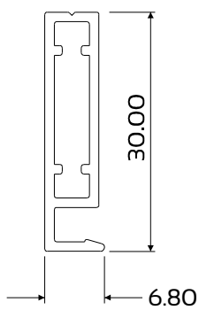
DIE No. W13484 Flyscreen Sash
