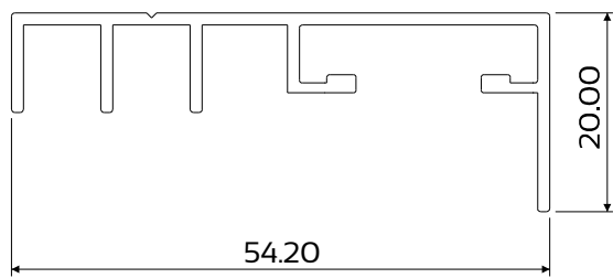
DIE No. W31069 Flyscreen Outer Frame
